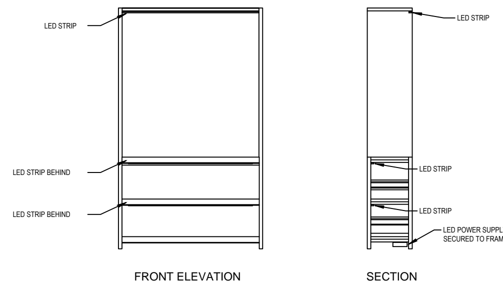
FRONT ELEVATION
