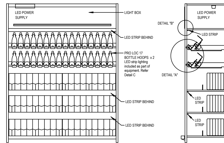
FRONT ELEVATION
