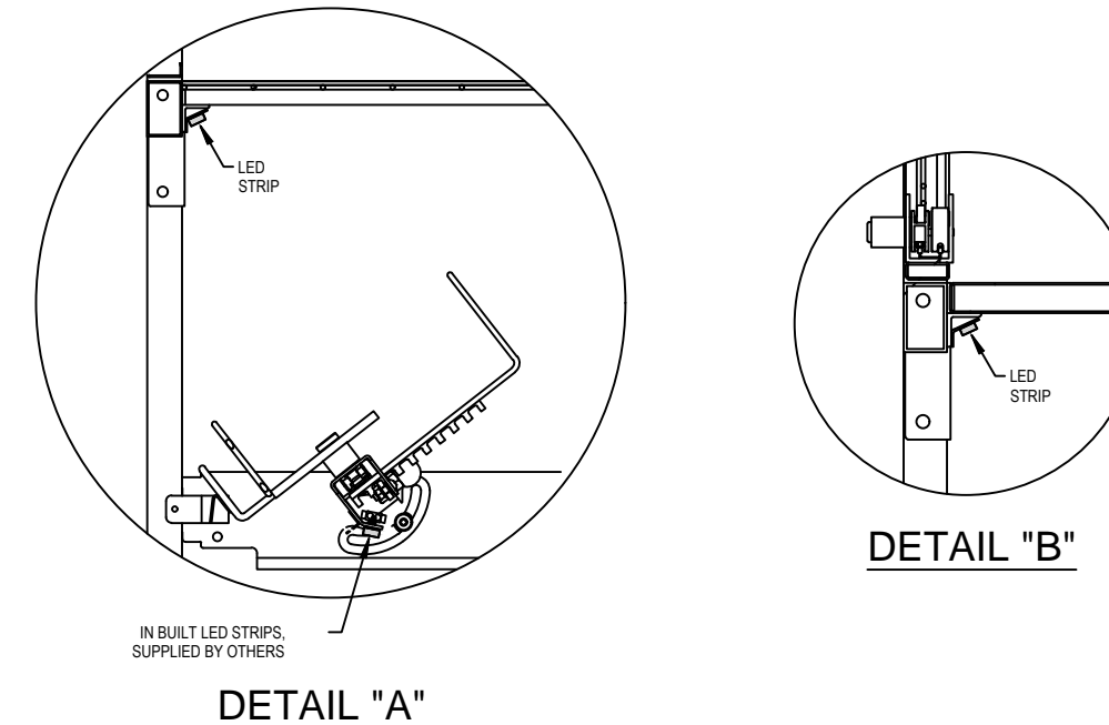
DETAIL "A"
