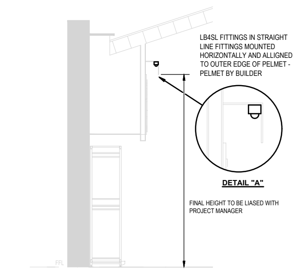
TYPICAL PELMET DETAIL
